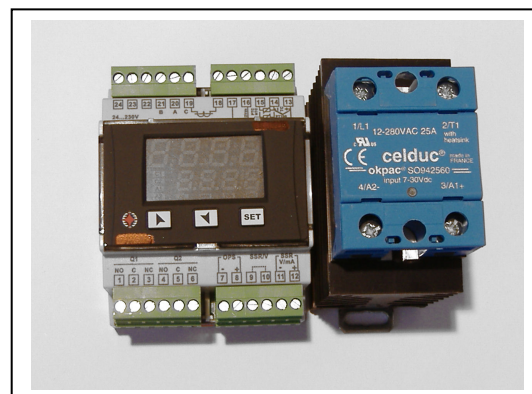
SMB-Standard controller 230V, SSR 25A and heat sink
